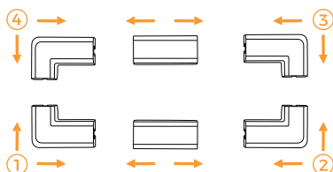
Mount L-shape fittings in pairs
